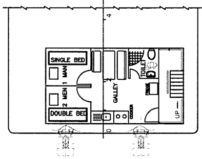
MAIN DECK
